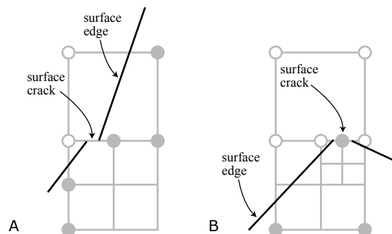
Figure 9. Adaptive grids can result in A) cracks in the surface edge which do not occur with the enhanced SurfaceNets algorithm and B) cracks in the surface edge which occur very rarely and can be prevented by a simple pre-conditioning step.
